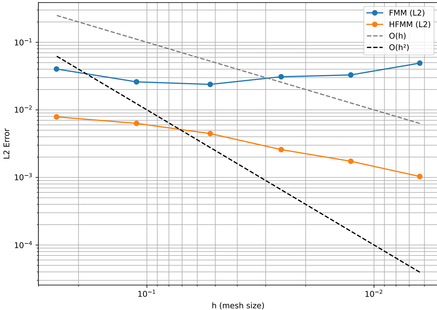
FMM Convergence - L-shape
